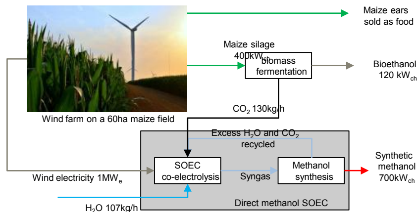
Figure 154: Direct methanol SOEC coupled with first generation bioethanol plant for land use optimization
