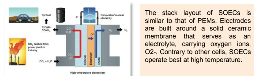
Figure 46: SOEC cell schematic and principle
