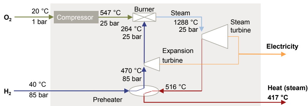
Figure 107: Schematic of a hydrogen turbine (left) 4 and illustration of a hydrogen turbine (right) 5
