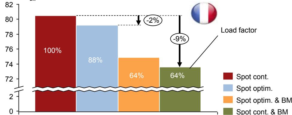
Figure 216: LCOH and load factor with balancing market strategies €/MWh ch
