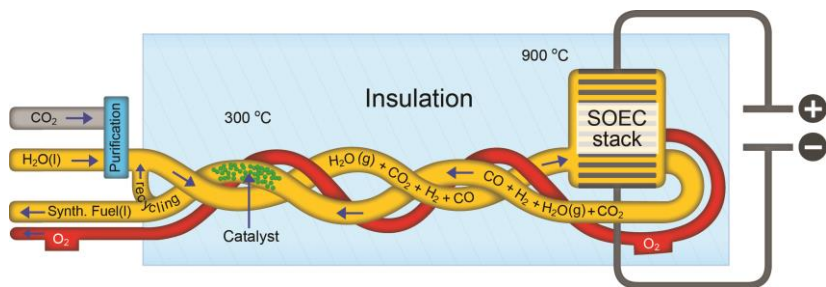
Figure 153: Direct synfuel SOEC stack
