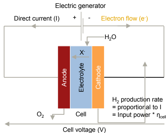
Figure 34: Schematic principle of a water electrolysis cell
