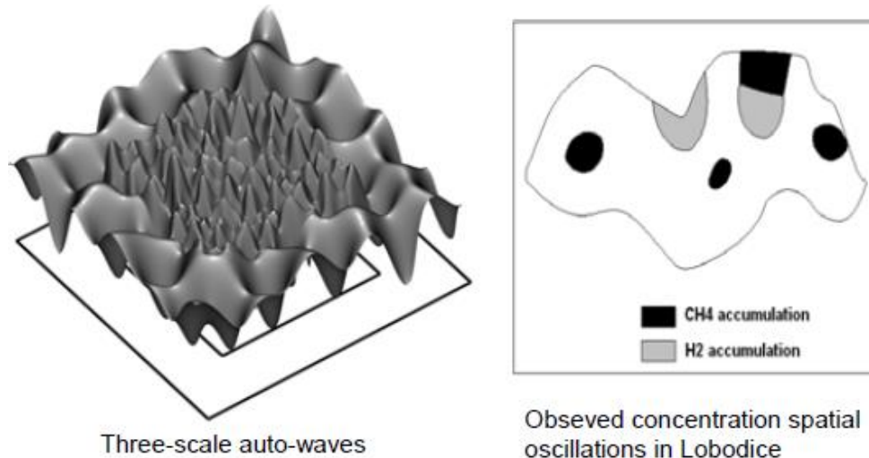
Figure 266: Heterogeneity of gases, resulting from bacterial methanogenesis 1
