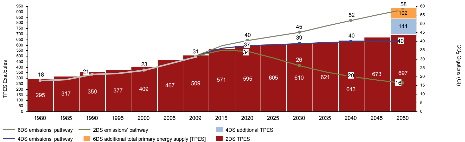
Figure 1: IEA CO 2 emissions and energy supply evolution, plus development pathways
