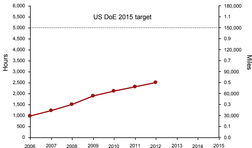
Figure 165: Mobile proton exchange membrane lifetime
