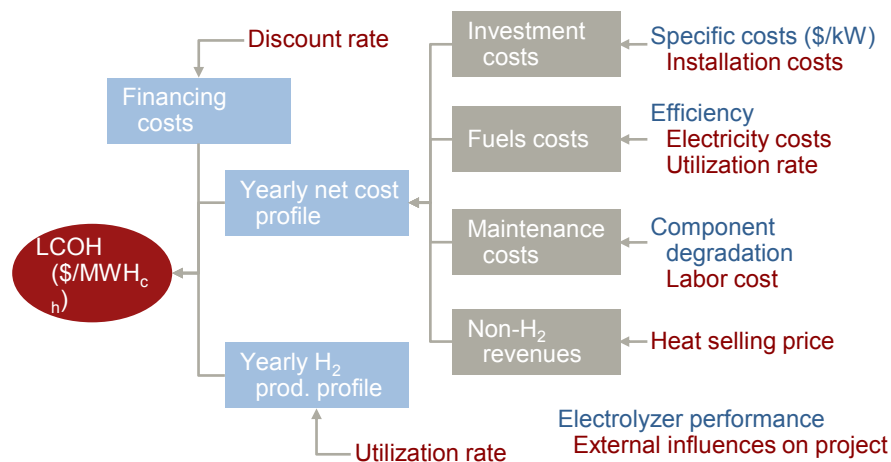
Figure 53: Levelized cost of hydrogen's impacting factors
