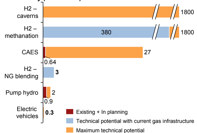
Figure 253: Potential for electricity storage system in Germany (ZFES 2012) 2 TWh
