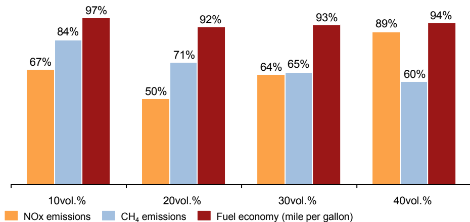
Figure 172: Comparative performances of different blends when running the motor at constant full load 1
