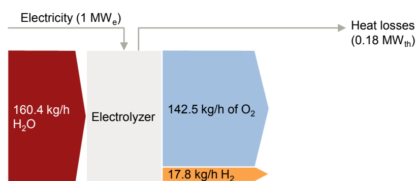
Figure 260: Flow chart of a typical commercial electrolyzer Electrogenics model 3
