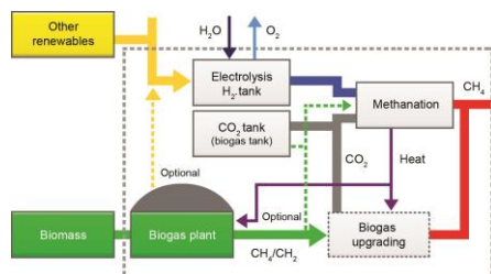
Figure 130: Electrolysis-assisted biomass plant layouts
